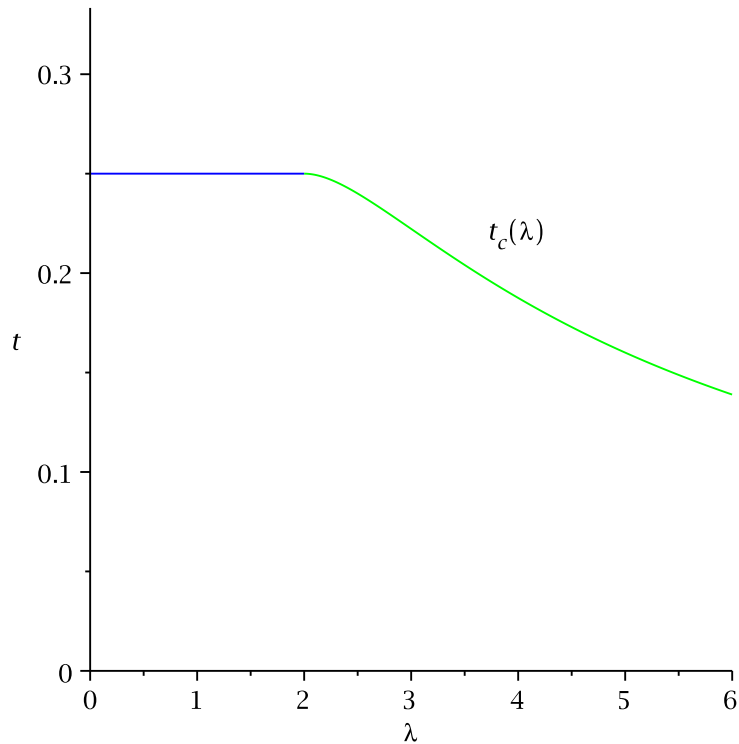
Figure 2: A plot of the radius of convergence t_c(\lambda) \equiv t_c(\lambda, 1) in the polymer length variable t of the generating function when q = 1 as a function of the force variable \lambda . Note that there is a change of behaviour at \lambda = 2 with constant t_c(\lambda) = 1/4 for \lambda \leq 2 .
