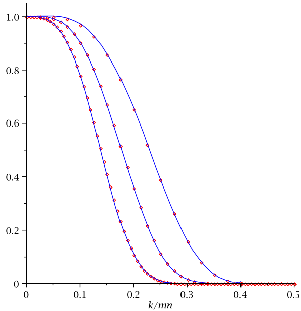
FIGURE 1. The probability p_{n,m,r}(k) that a word with k errors has a correctible error pattern versus the error frequency k/mn for C_m wr S_n , when m = 5 (and thus r = \lfloor \frac{5-1}{2} \rfloor = 2 ). Shown is a comparison of the exact values (shown as points) and the asymptotic result (shown as curves) from Proposition 13 for n = 8, 16 , and 32 (from right to left).
