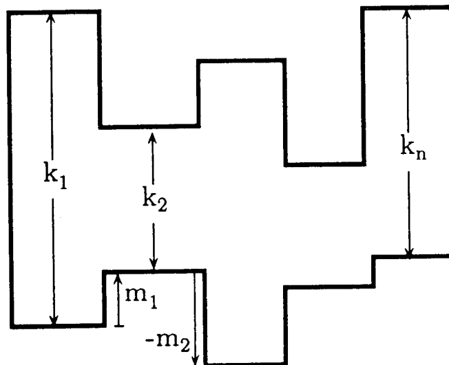
Fig. 5. Length labeling of the lattice column-convex model.
