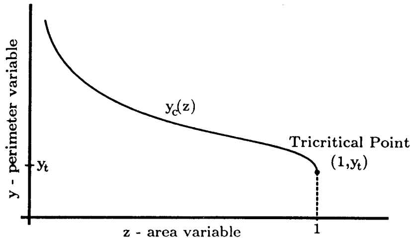
Fig. 2. Schematic plot of the radius of convergence of the generating function showing the tricritical point.
