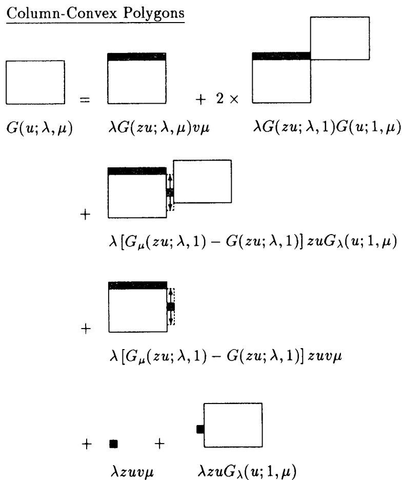
Fig. 4. Diagrammatic form of the functional equation. The clear square corresponds to the generating function G , the black regions are parts added to G . The arrows indicate summation over the height of the indicated region.
