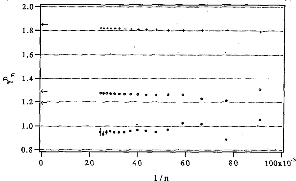
Figure 2. This graph is a plot of local estimates of the exponent \gamma^D against 1/n for the three temperatures. The crosses are high temperatures values, the open circles are \theta -temperature values and the full circles are the low temperature values. The arrows indicate the conjectured results. At low temperatures the estimates are more erratic than at high temperatures though they still settle to a value well away from the conjectured 19/16 .
