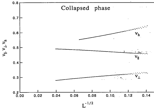
FIG. 13. The low-temperature ( \omega=6.0 ) length-scale exponents can be estimated from this plot of \nu_{\parallel} , \nu_{\perp} , and \nu_h . Here the corrections to scaling should be of order L^{-1/2} . A 600-term series was used.
