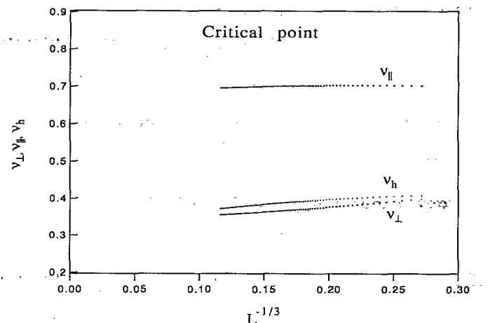
FIG. 12. The critical-temperature ( \omega = 3.382975 \dots ) length-scale exponents can be estimated from this plot of \nu_{\parallel} , \nu_{\perp} , and \nu_h . Here the corrections to scaling should be of order L^{-1/3} . A 600-term series was used.
