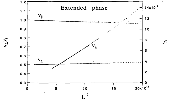
FIG. 11. The high-temperature ( \omega = 1.0 ) length-scale exponents can be estimated from this plot of \nu_{\parallel} , \nu_{\perp} , and \nu_h . The corrections should be of order L^{-1} (from the exact solution) and so we use this as the variable against which we plot. A 600-term series was used here because of the greater complexity of the series needed to calculate length-scale exponents.
