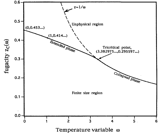
FIG. 3. The singularity diagram for the discrete IPDSAW model. Important points, including free walks at \omega=1 and the tricritical collapse point, are shown.
