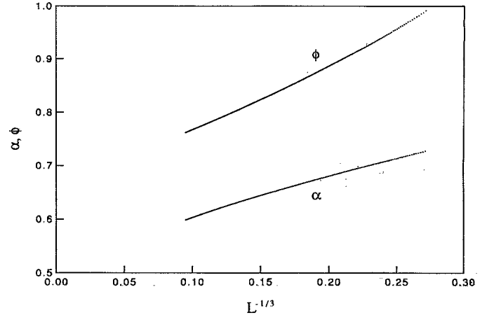
FIG. 4. Estimates for the exponents \alpha and \phi at the collapse transition are plotted against a corrections-to-scaling term of L^{-1/3} for L up to 2000. The exact values are \frac{1}{2} and \frac{2}{3} , respectively. This plot shows that the series are only slowly convergent.
