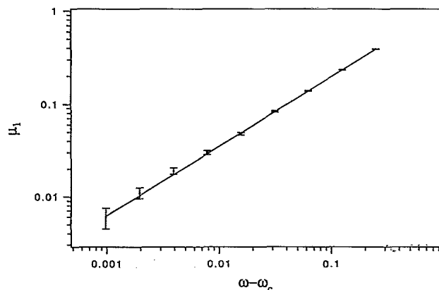
FIG. 10. To provide an estimate for the exponent \chi , a log-log plot of \mu_1 is given against the "temperature" difference to the critical point ( \omega - \omega_c ). A 6000-term series was used to calculate \mu_1 . The straight line has slope \frac{3}{4} .
