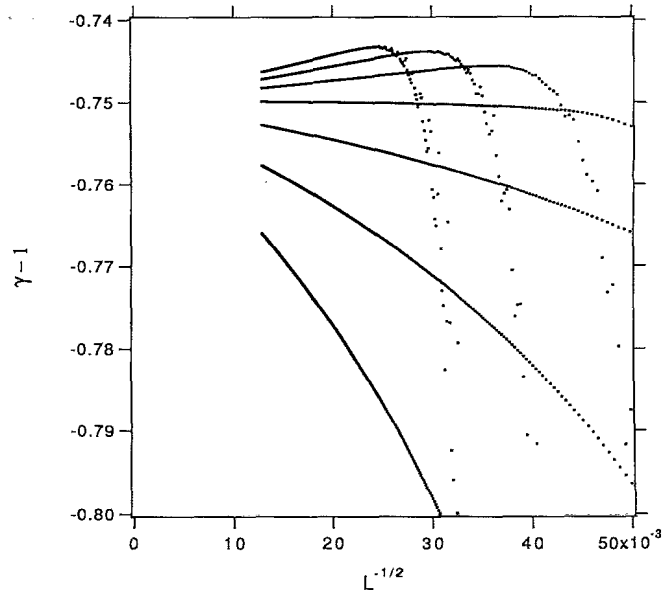
FIG. 2. Estimates for the exponent \gamma - 1 fitting the calculated partition function by the full form (3). Again these cover the same range of temperatures as in Fig. 1, from top to bottom (on the left-hand side). Fitting these curves with third- and fourth-order polynomials in l^{-1/2} produces remarkably stable results.
