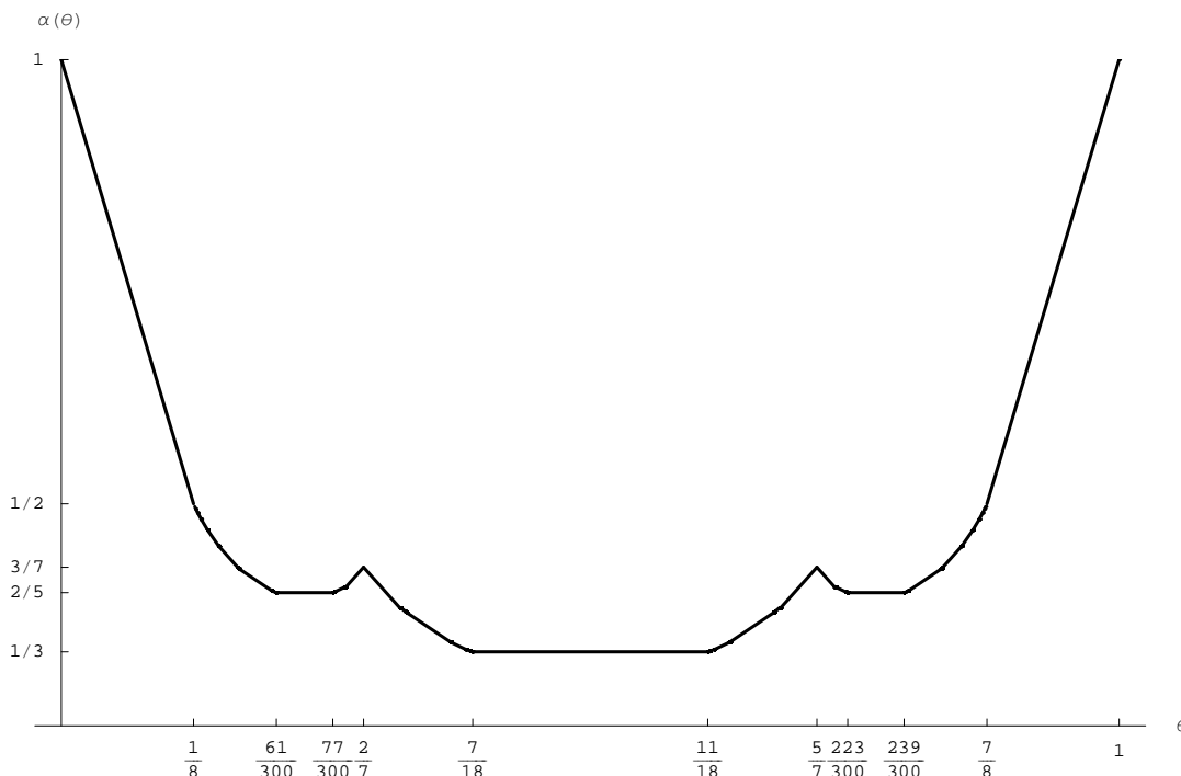
FIGURE 4. Graph of the countably piecewise affine function \alpha(\theta) := \max_{\mu \in \mathcal{M}} \int f_\theta d\mu . Only 9 of its 23 intervals of monotonicity are visible.
