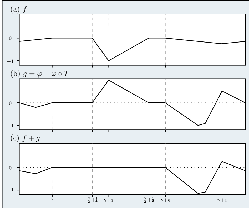
FIGURE 3. Flattening of the function f from Example 4.12: f itself is shown in (a), the unique Lipschitz coboundary g = \varphi - \varphi \circ T flattening f on the one-flower F = [\lambda, \lambda + 1/2] is shown in (b), and the flat function f + g is shown in (c). Although flat on F , the function f + g is not in normal form as its maximum (at \gamma + 3/4 ) is larger than 0. The function f is in normal form; the unique Sturmian measure carried by F is also carried by the set of maxima of f , so is the unique f -maximizing measure. Thus f may be flattened on F (i.e. satisfies the pre-Sturmian condition), but the corresponding flat function is not in normal form, so f does not satisfy the Sturmian condition, even though its maximizing measure is Sturmian.
