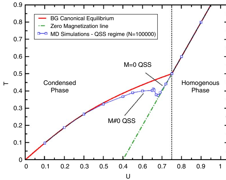
Fig. 1. In this figure we plot—for N = 100\,000 —the molecular dynamics numerical results corresponding to QSS (open squares), compared with both the canonical caloric curve, plotted as solid line, and the zero magnetization (or minimum temperature) line, reported as dot-dashed. The temperature is calculated by means of the average kinetic energy K , i.e. T = 2K/N . The QSS follows the latter line only up to U = 0.68 , becoming unstable below this limiting value [20,41].
