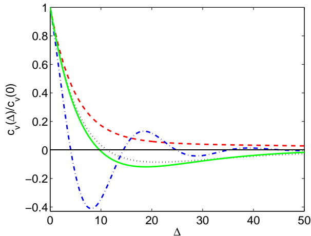
FIG. 1: (Colour online) Plot of the correlation function for different values of \sigma . The solid line is a representation of expression (19), i.e. the case B = 0 . The dashed-dotted curve shows an oscillatory behavior (20). The dashed and dotted curve are respectively a sum and difference of two exponential functions (21).
