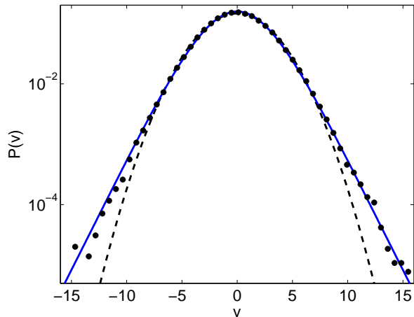
FIG. 2: (Colour online) Plot of the measured distribution P(v) ( \bullet\bullet\bullet ). The dashed line represents a Gaussian approximation 0.15 \exp(-0.07v^2) for P(v) . The solid line is the superstatistical distribution (3), with f(\beta) a lognormal distribution (22).
