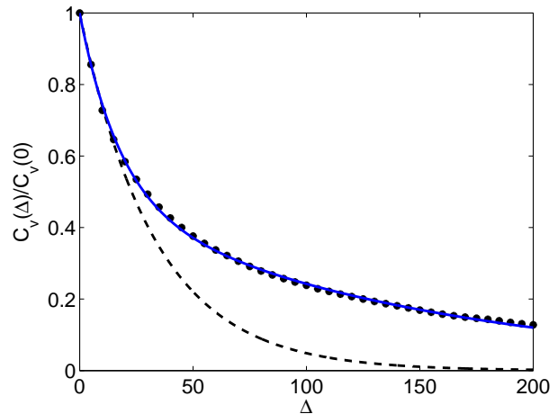
FIG. 3: (Colour online) Plot of the measured normalised correlation function C_v(\Delta)/C_v(0) ( \bullet\bullet\bullet ). The dashed and solid lines represent an approximation for C_v(\Delta)/C_v(0) in terms of a single exponential \exp(-0.030\Delta) and a sum of two exponentials (21), respectively.
