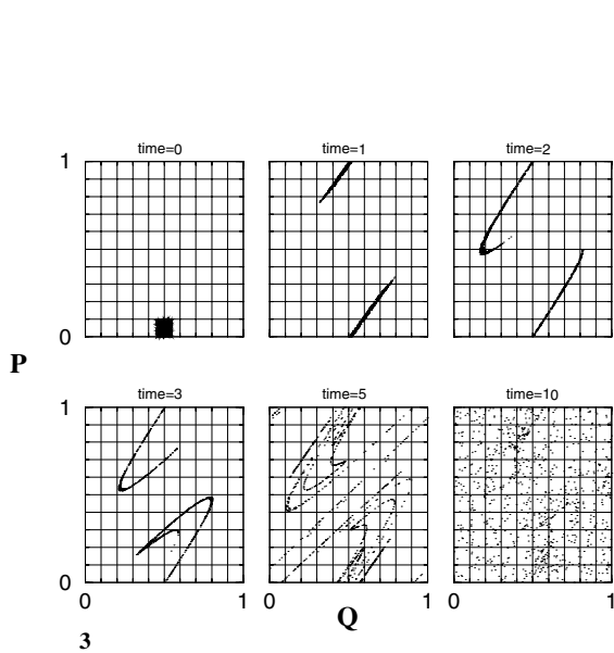
Fig. 3. Standard map with a = 5 . Time evolution of an initial distribution of points; we report time = 0, 1, 2, 3, 5, 10.
