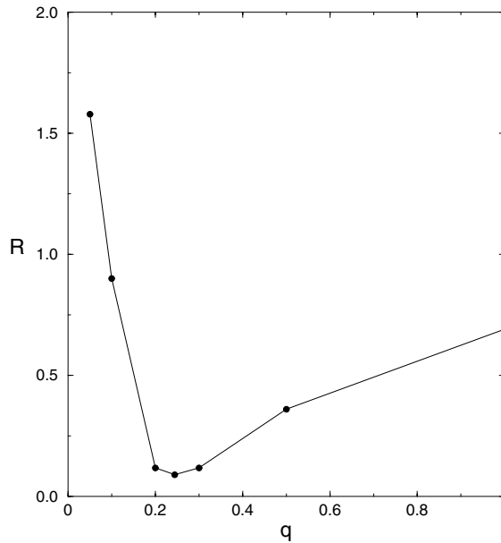
Fig. 9. Coefficient of nonlinearity R vs. q . See text for further details.
