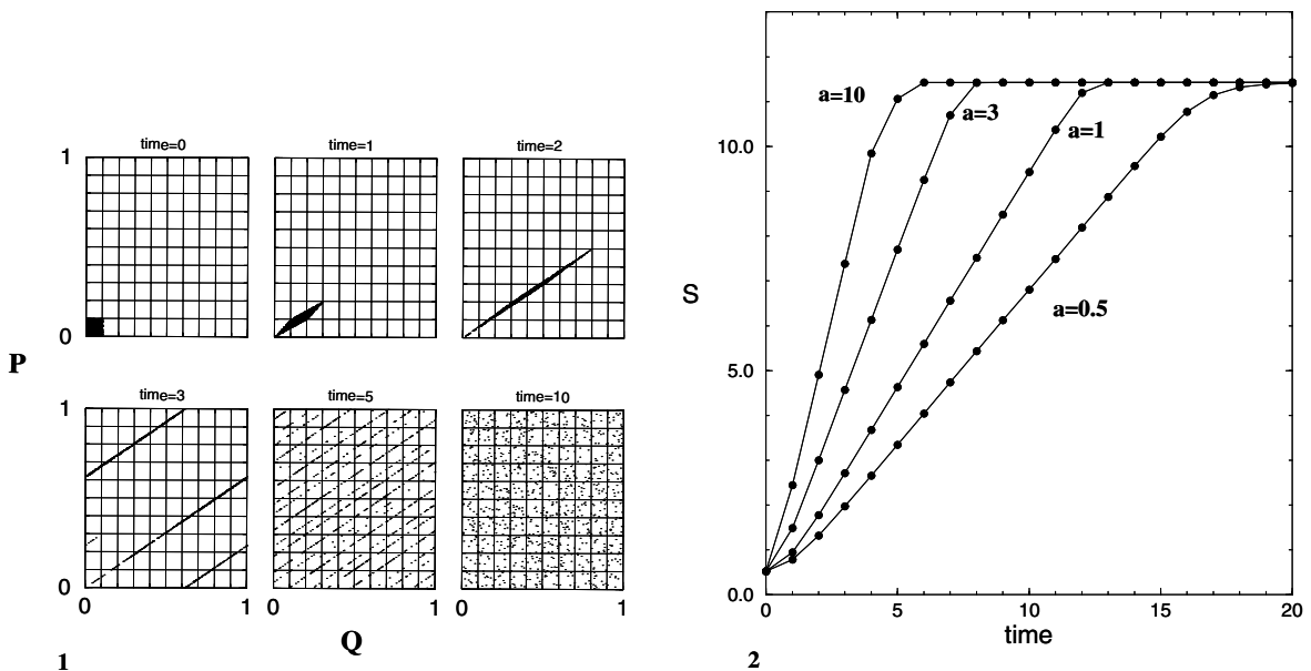
Fig. 1. Generalized cat map with a = 1 . Time evolution of an initial distribution of points; we report the following time steps 0,1,2,3,5,10.
